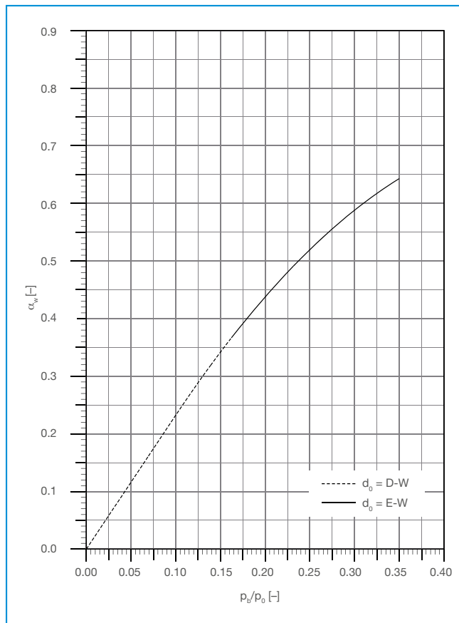
Si 830 coefficient of discharge \alpha_w depending on p_b/p_0 for liquid
