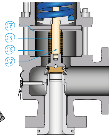
Bellows design Si 84
