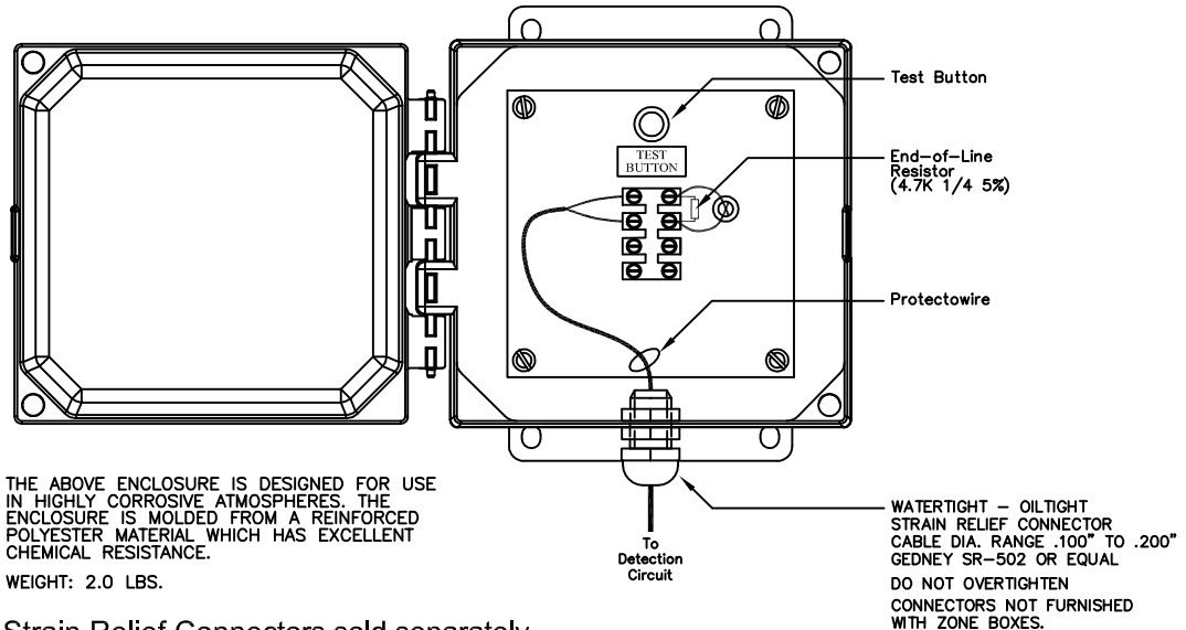
MOUNTING PANEL DETAIL 4.81" x 4.81" (122.24mm) x (122.24mm) MOUNTED INSIDE OF CABINET
